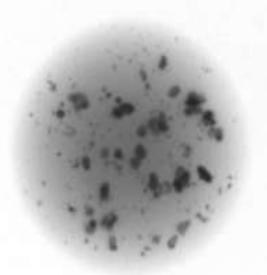
TEM-image of a dried acrylate spray droplet from a propellant spray can with embedded ZnO additive particles and TiO 2 pigment particles.
